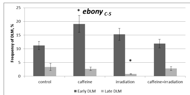
Fig. 3. Frequency of early and late DLM mutant line ebony C-S after the action of physical and chemical factors.
